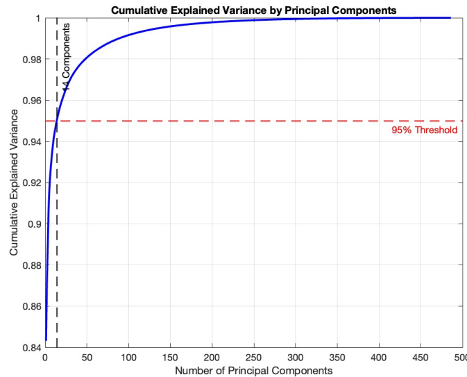
Figure 3: Cumulative Explained Variance for different PC's
