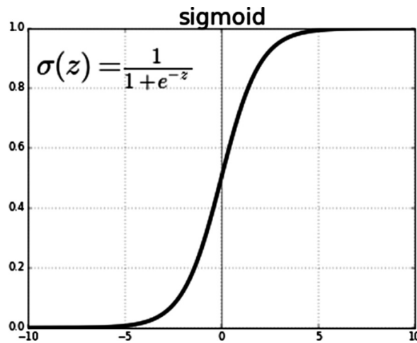
Figure 45: Sigmoid Function
